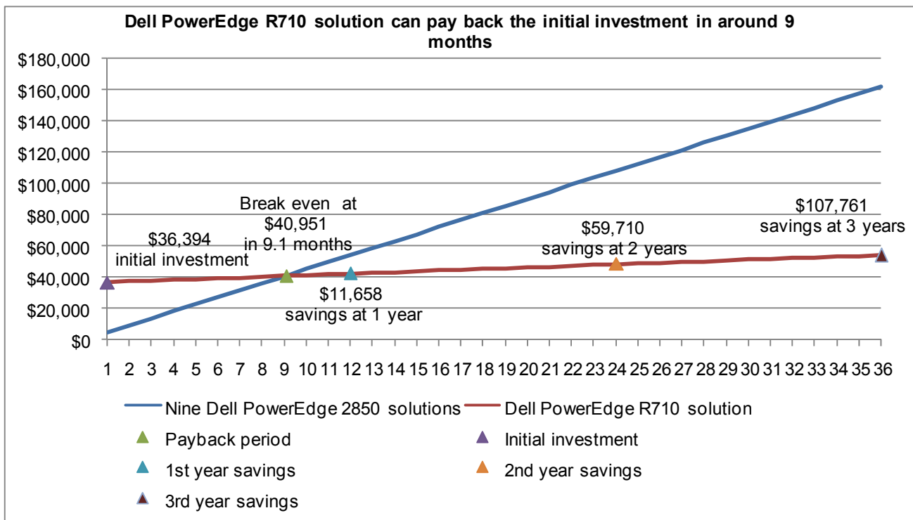
Figure 2: The payback period and cumulative estimated costs 1 for the nine Dell PowerEdge 2850 solutions and the Dell PowerEdge R710 solution. Lower costs and higher savings are better.
